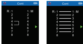
Short circuit of cores 4 and 5
