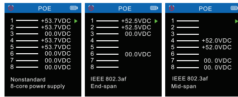
8-core power supply, 53.7V
